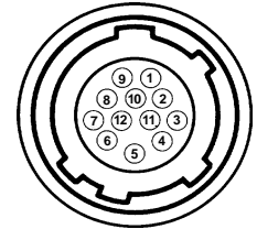
7 Front view of receptacle on RPS-77
