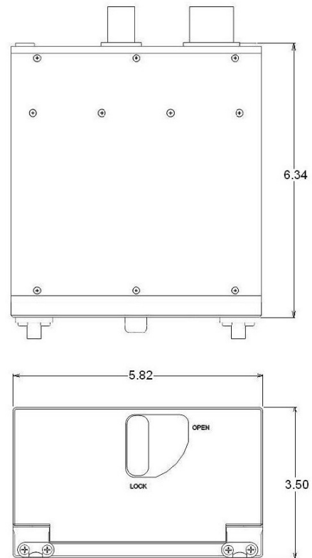
Sekai ADV-D2 Dimensions
