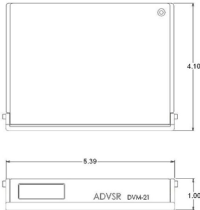
Sekai DVM-21 Dimensions
